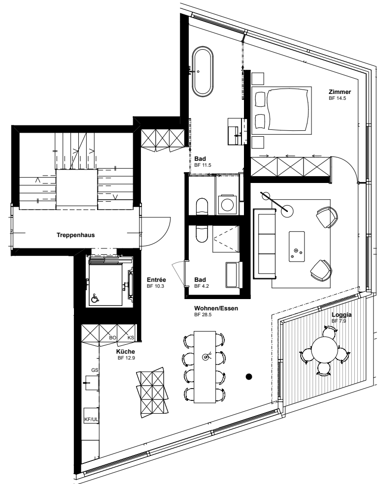
WHG 1.22 EG Haus 1, 2.5 Zi
